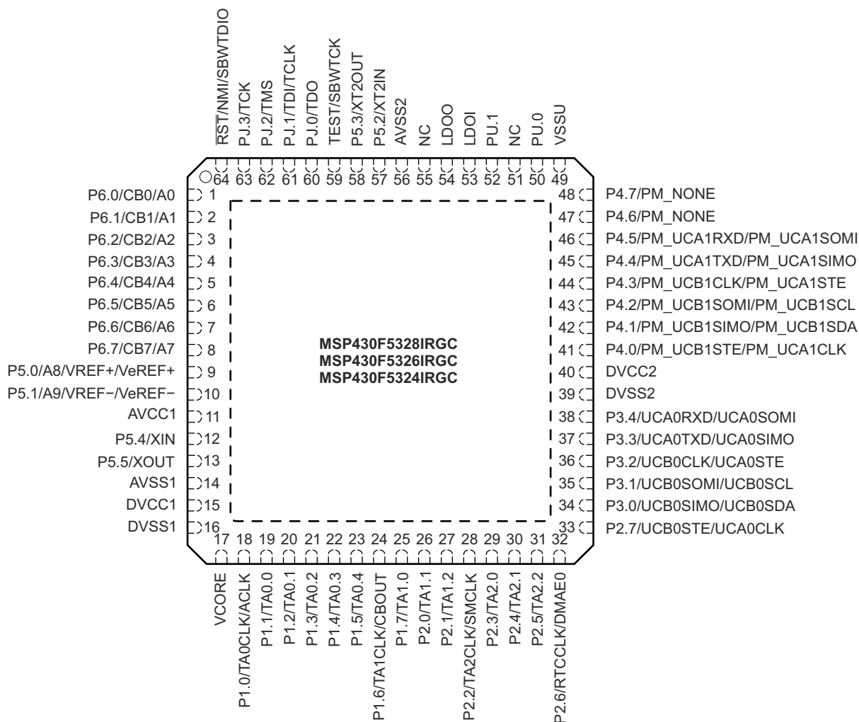
Figure 7-2. 64-Pin RGC Package (Top View) – MSP430F5328IRGC, MSP430F5326IRGC, MSP430F5324IRGC
