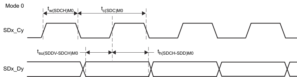
Figure 6-84. SDFM Timing Diagram – Mode 0
