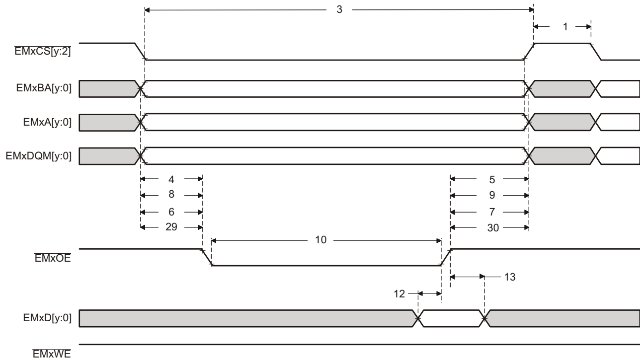
Figure 6-43. Asynchronous Memory Read Timing
