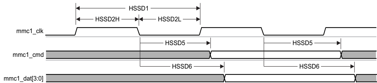
Figure 5-81. MMC/SD/SDIO in - High Speed - Transmitter Mode
