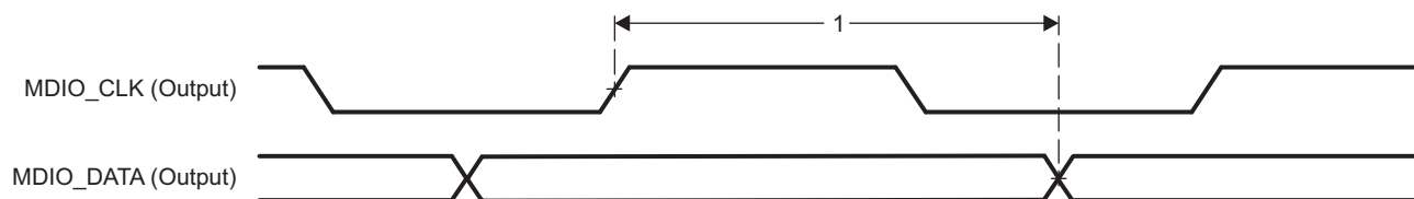
Figure 5-124. PRU-ICSS MDIO_DATA Timing – Output Mode
