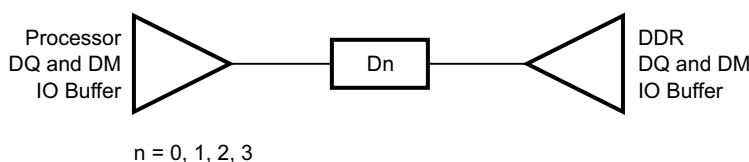
Figure 7-59. DQ/DM Topology
