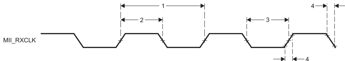
Figure 5-125. PRU-ICSS MII[x]_RXCLK Timing
