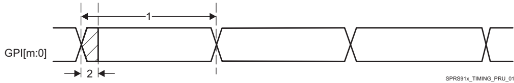
Figure 5-109. PRU-ICSS PRU Direct Input Timing
