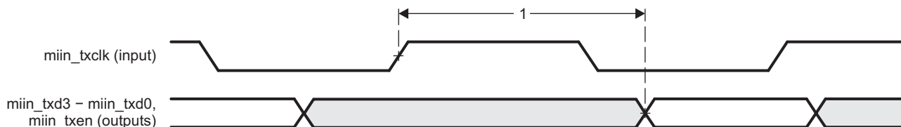
Figure 5-71. GMAC Transmit Interface Timing MIIn Operation
