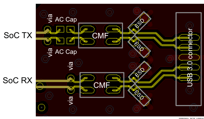
Figure 7-40. USB 3.0 placement diagram
