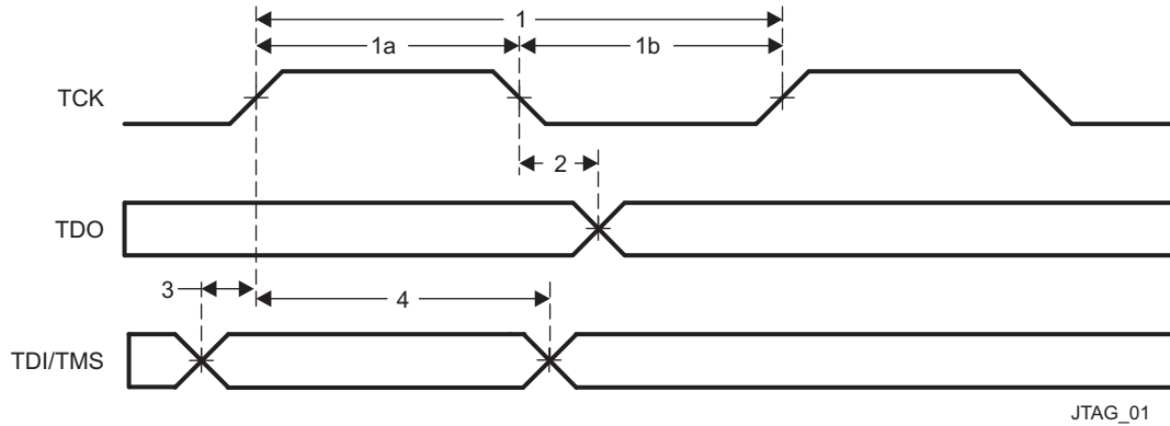
Figure 5-110. JTAG Timing
