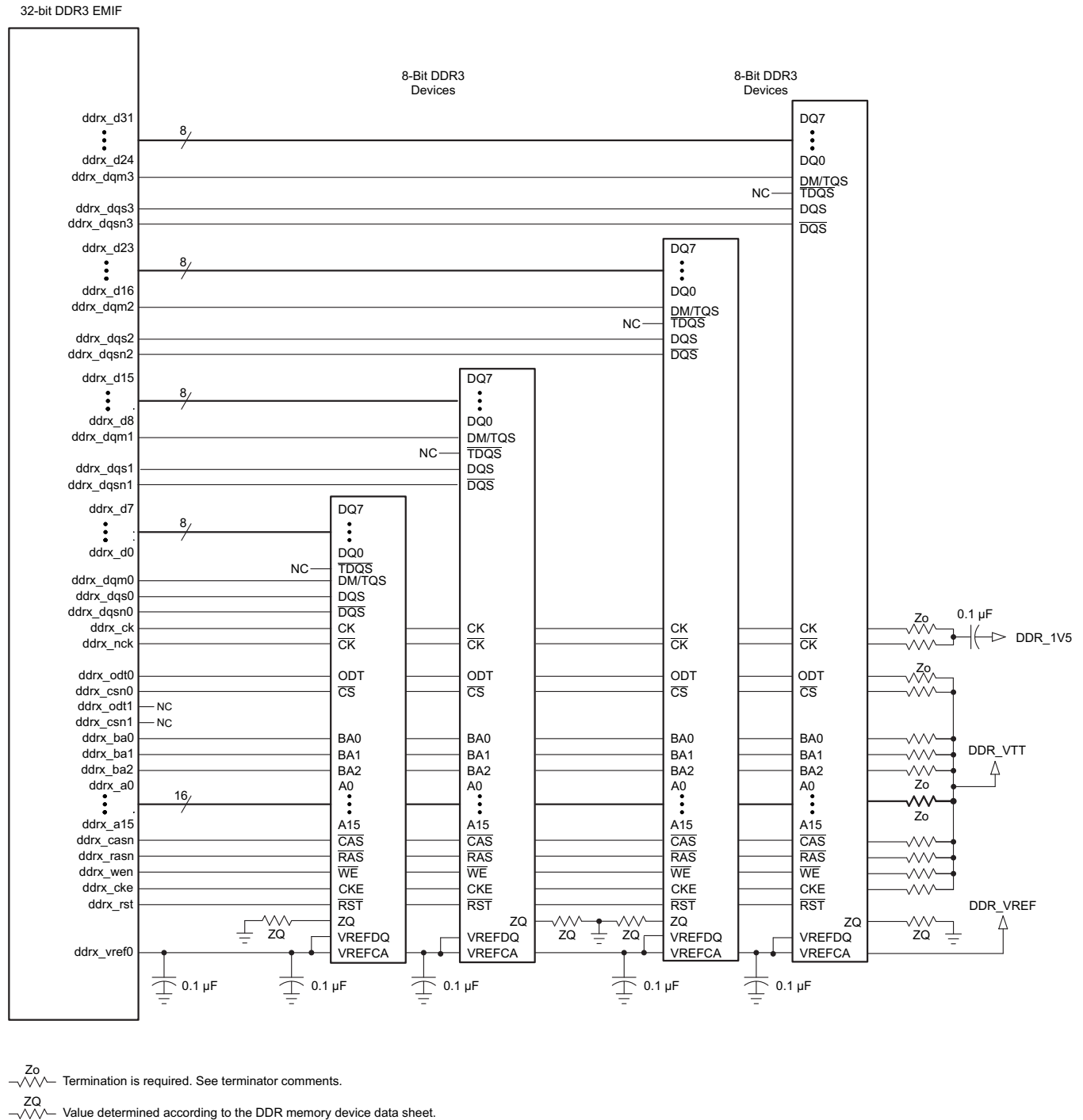
Figure 7-56. 32-Bit, One-Bank DDR3 Interface Schematic Using Four 8-Bit DDR3 Devices
