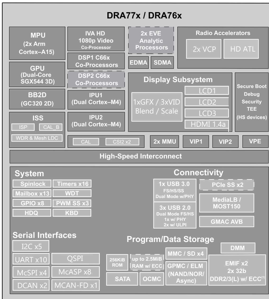
Figure 6-1. DRA77x, DRA76x Block Diagram
