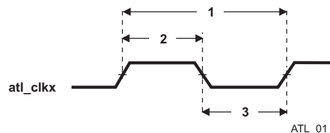
Figure 5-109. ATL_CLKOUTx Timing
