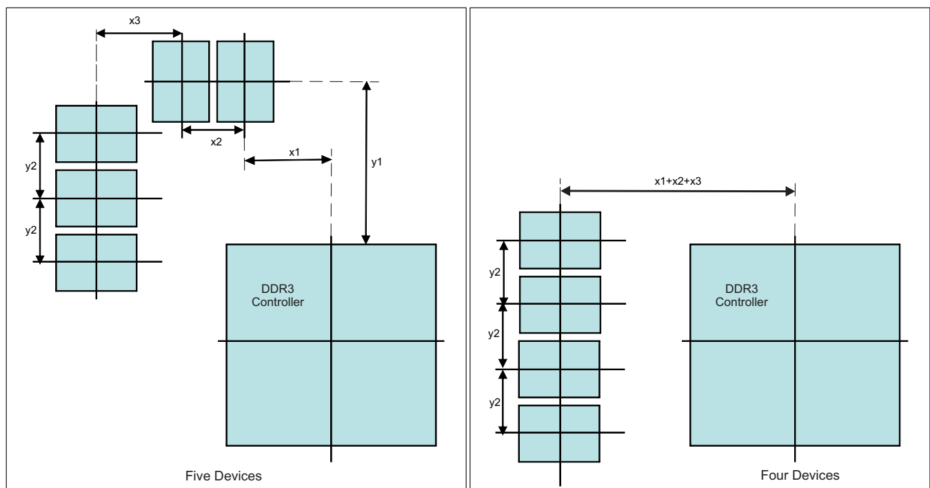
Figure 7-57. Placement Specifications
