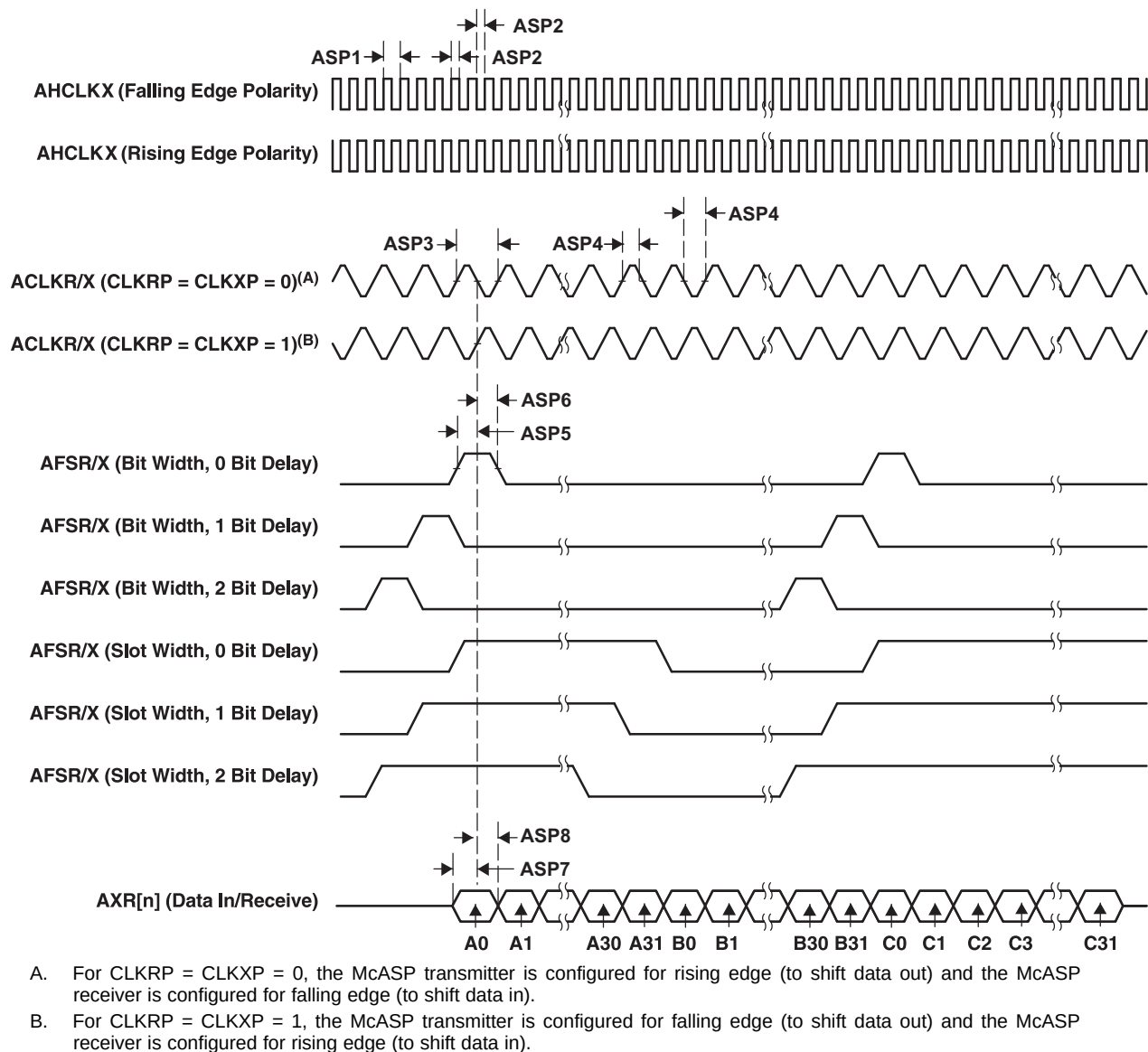
Figure 5-57. McASP Input Timing
