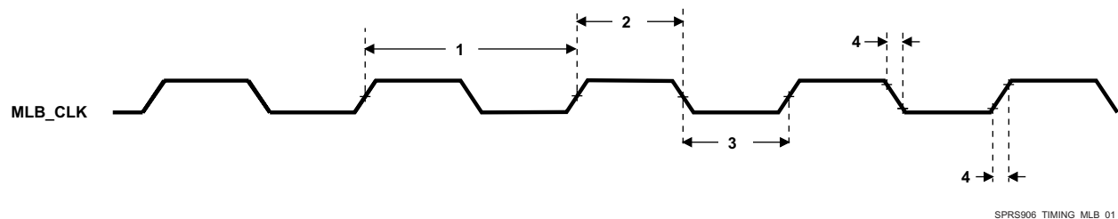
Figure 5-77. MLB_CLK Timing
