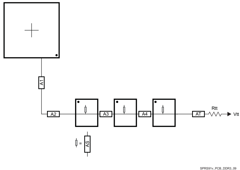
Figure 7-52. ADDR_CTRL Routing for Three Single-Side DDR3 Devices
