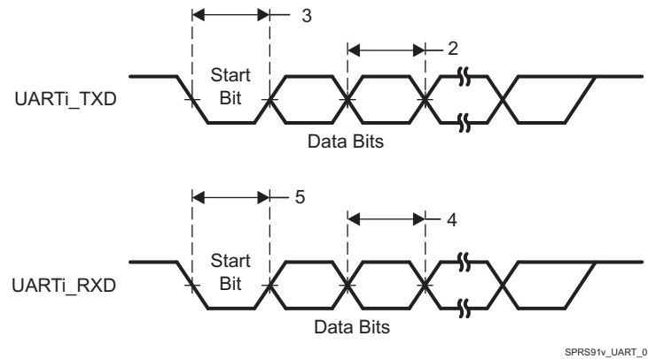
Figure 5-40. UART Timing
