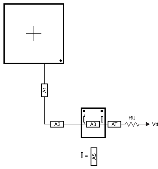
Figure 7-59. CK Routing for Two Mirrored DDR3 Devices
