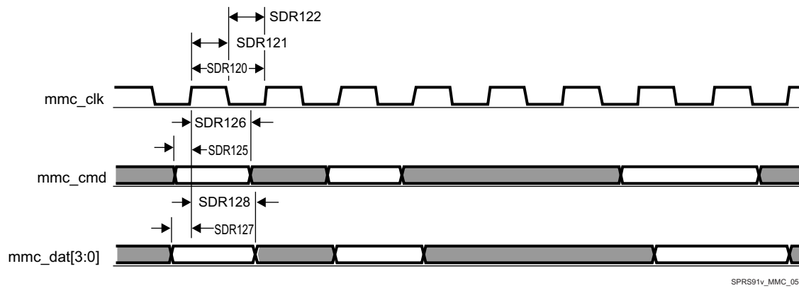
Figure 5-58. MMC/SD/SDIOj in - SDR12 - Receiver Mode
