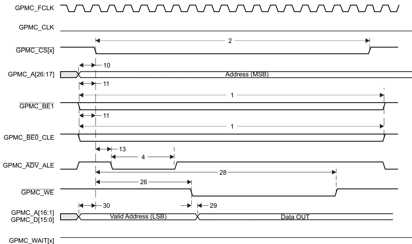
Figure 8-32. GPMC/Multiplexed NOR Flash - Asynchronous Write - Single Word Timing
