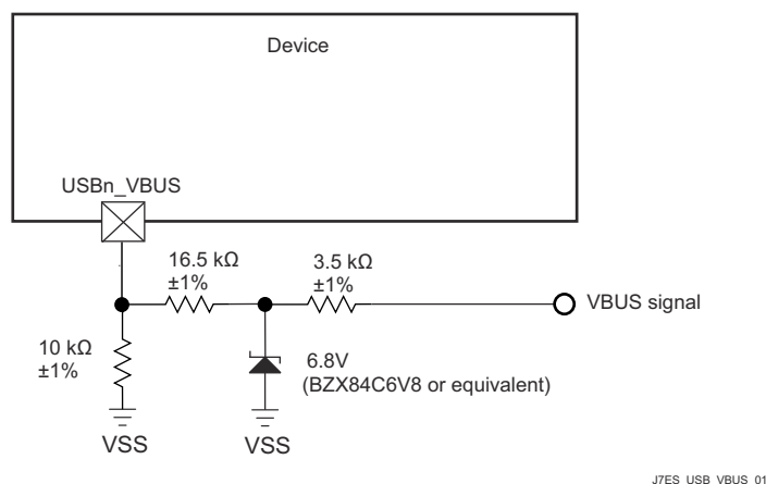
Figure 9-4. USB VBUS Detect Voltage Divider / Clamp Circuit
