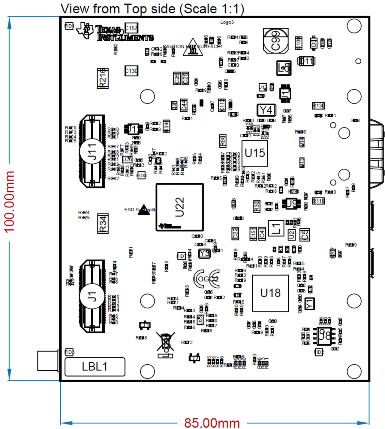
Figure 8-4. AM273x EVM - Top Assembly
