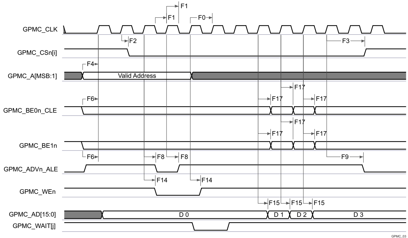
Figure 6-38. GPMC and NOR Flash — Synchronous Burst Read — 4x16-bit (GPMCCLKDIVIDER = 0)
