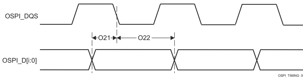
Figure 6-79. OSPI0 Timing Requirements – PHY SDR with External Board Loopback
