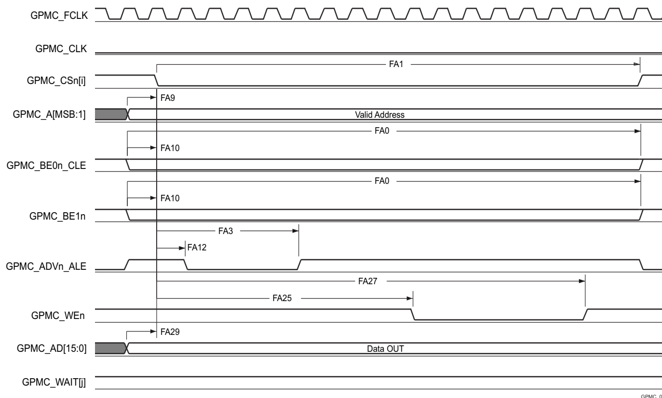
Figure 6-45. GPMC and NOR Flash — Asynchronous Write — Single Word
