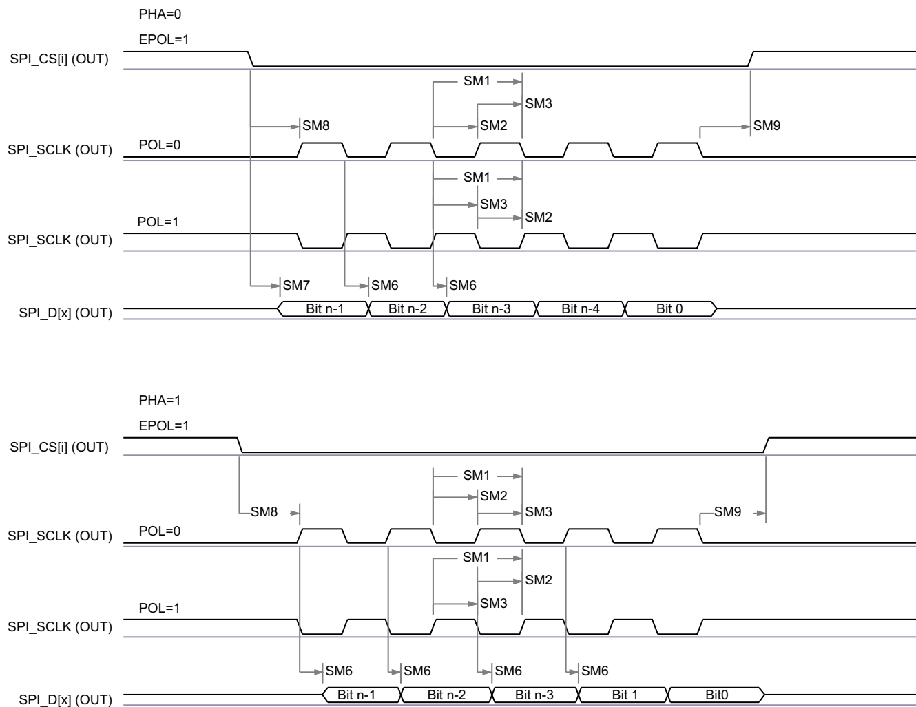
Figure 6-53. MCSPI Controller Mode Transmit Timing
