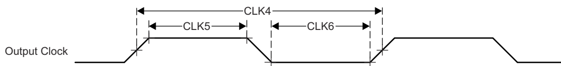
Figure 6-13. Clock Switching Characteristics
