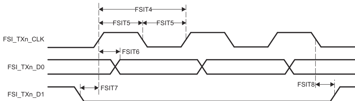
Figure 6-36. FSI Switching Characteristics - SPI Mode
