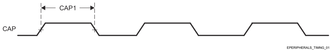
Figure 6-27. ECAP Timings Requirements
