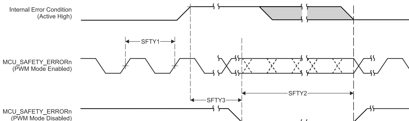
Figure 6-11. MCU_SAFETY_ERRORn Timing Requirements and Switching Characteristics
