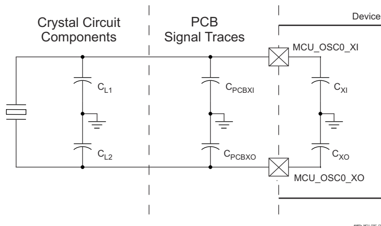
Figure 6-17. Load Capacitance
