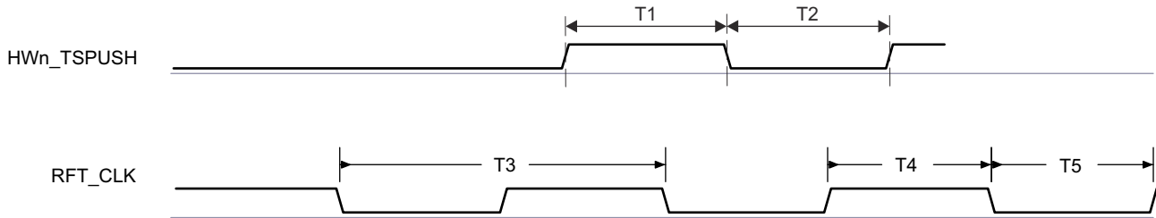
Figure 6-74. CPTS Timing Requirements
