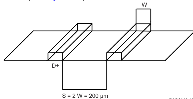
Figure 8-1. Ground Guard Illustration
