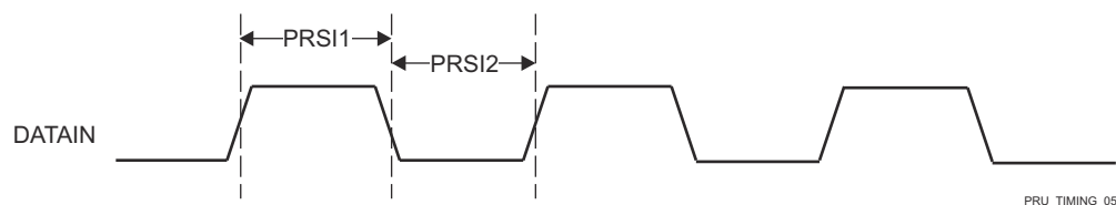
Figure 6-90. PRU_ICSSG PRU Shift In Timing
