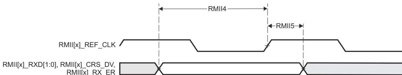
Figure 6-22. CPSW3G RMII[x]_RXD[1:0], RMII[x]_CRS_DV, RMII[x]_RX_ER Timing Requirements – RMII Mode
