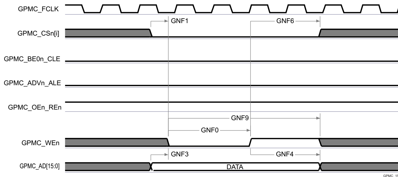
Figure 6-51. GPMC and NAND Flash — Data Write Cycle
