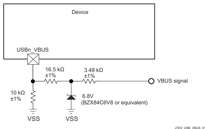
Figure 8-5. USB VBUS Detect Voltage Divider / Clamp Circuit
