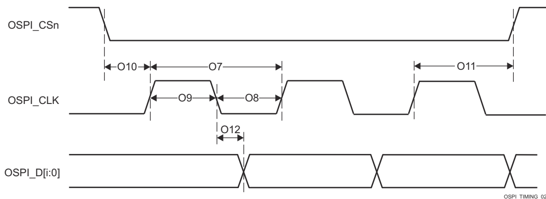
Figure 6-80. OSPI0 Switching Characteristics – PHY SDR
