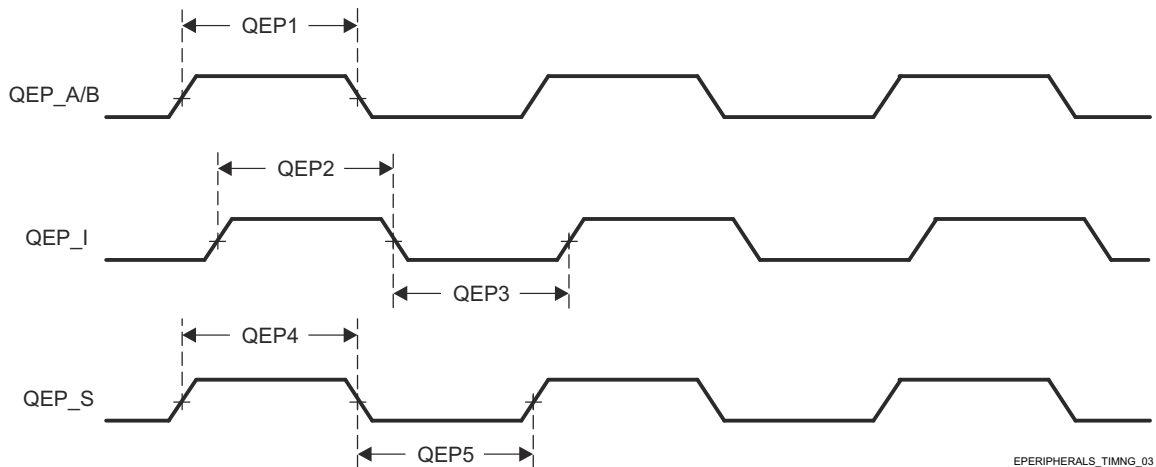
Figure 6-33. EQEP Timing Requirements
