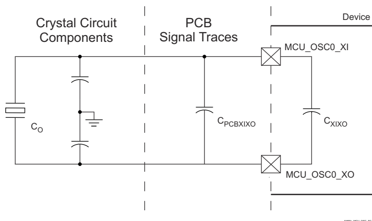
Figure 6-18. Shunt Capacitance
