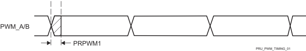
Figure 6-96. PRU_ICSSG PWM Timing
