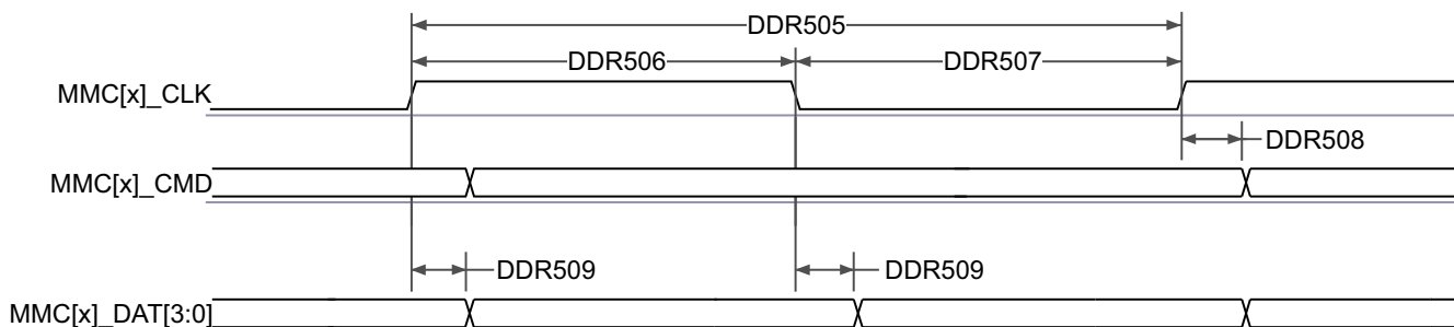
Figure 6-72. MMC1 – UHS-I DDR50 – Transmit Mode
