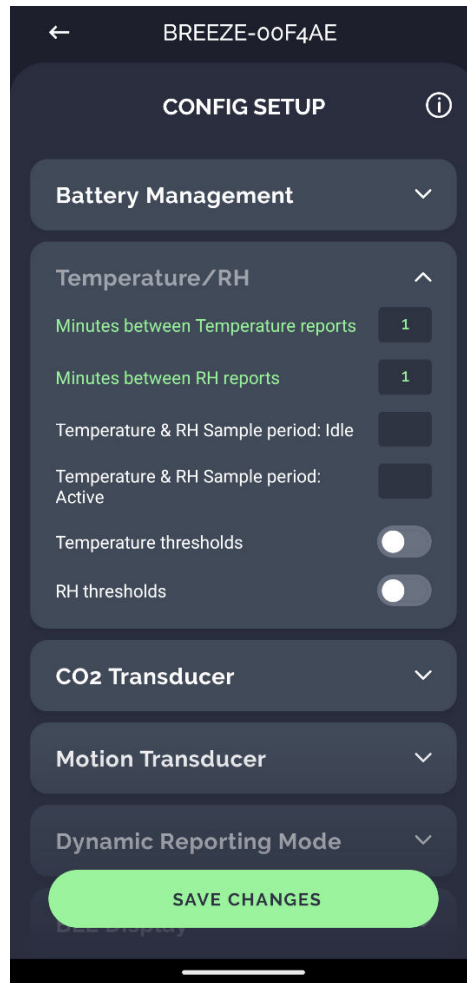
Figure 9 LeapX application
