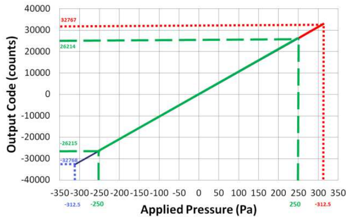
SM933X-250 Pa: Count vs. Pressure
