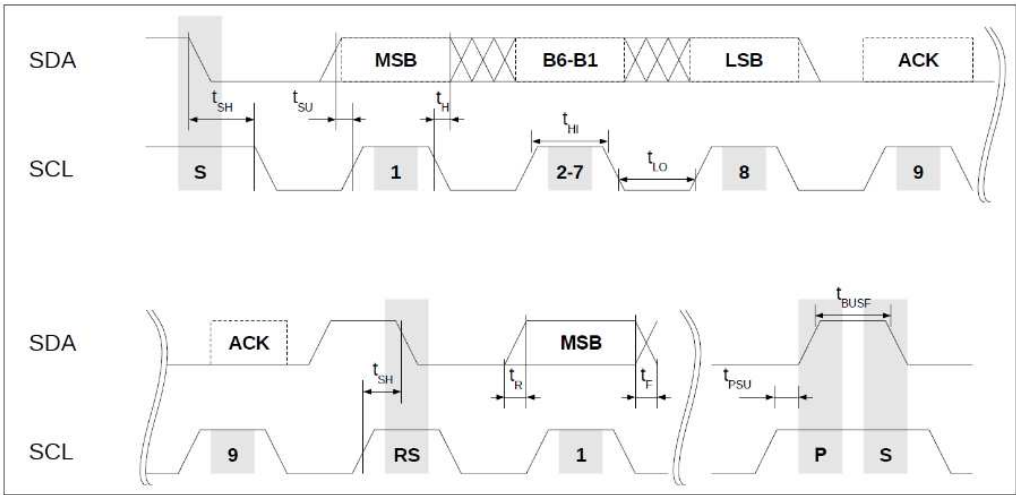
I 2 C Interface Timing Diagram:
