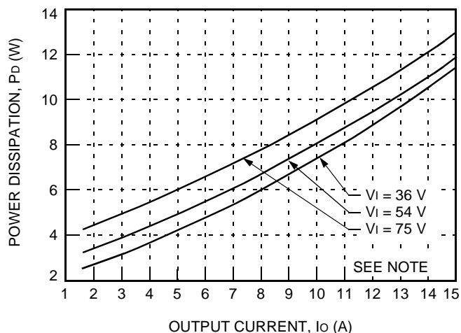
Figure 24. QW075F1 Power Dissipation vs. Output Current at Room Temperature
