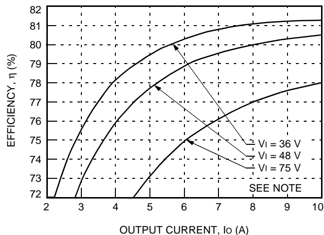
Figure 3. Typical QW050F1 Converter Efficiency vs. Output Current at Room Temperature
