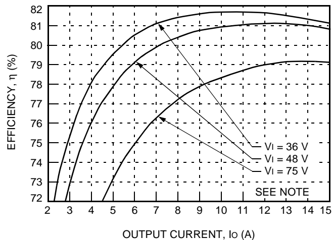
Figure 4. Typical QW075F1 Converter Efficiency vs. Output Current at Room Temperature
