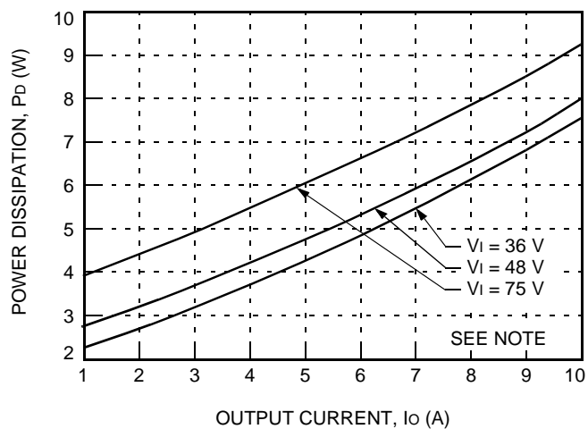
Figure 23. QW050F1 Power Dissipation vs. Output Current at Room Temperature
