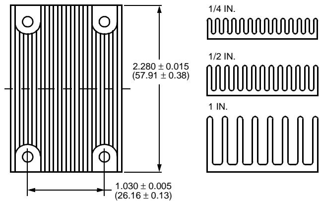
Figure 33. Longitudinal Heat Sink
