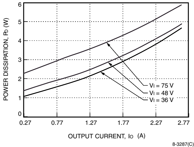
Figure 14. QW030C Typical Power Dissipation vs. Output Current at T_A = 25^\circ\text{C}
