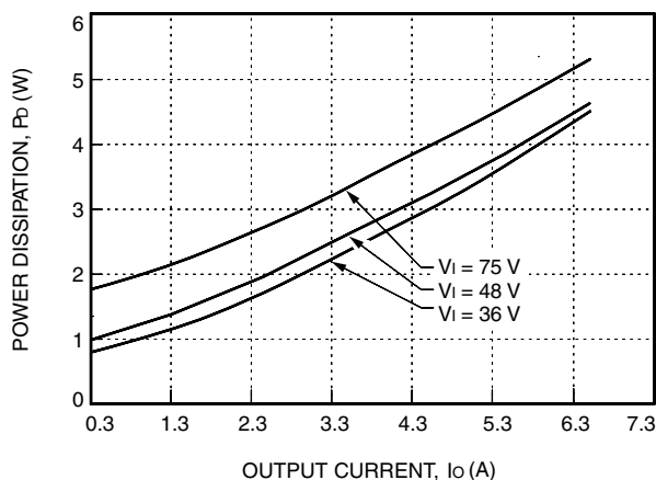
Figure 11. QW030F Typical Power Dissipation vs. Output Current at T_A = 25^\circ\text{C}
