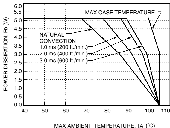
Figure 10. QW030B, C Forced Convection Power Derating with No Heat Sink; Either Orientation
