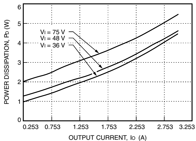
Figure 13. QW030B Typical Power Dissipation vs. Output Current at T_A = 25^\circ\text{C}
