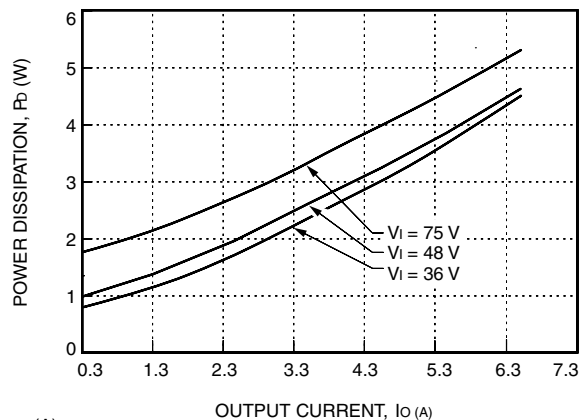
Figure 12. QW030A Typical Power Dissipation vs. Output Current at T_A = 25^\circ\text{C}
