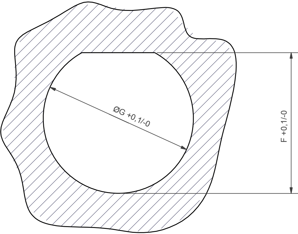
PANEL CUTOUT
