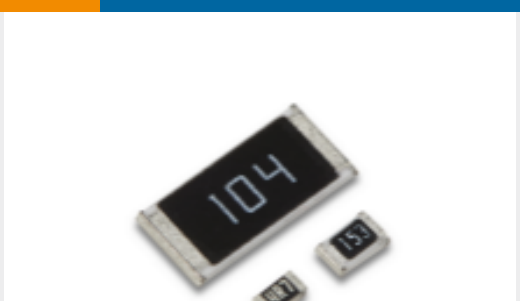
TE Part #1-2176349-6 CRGCQ 2512 180R 1%
