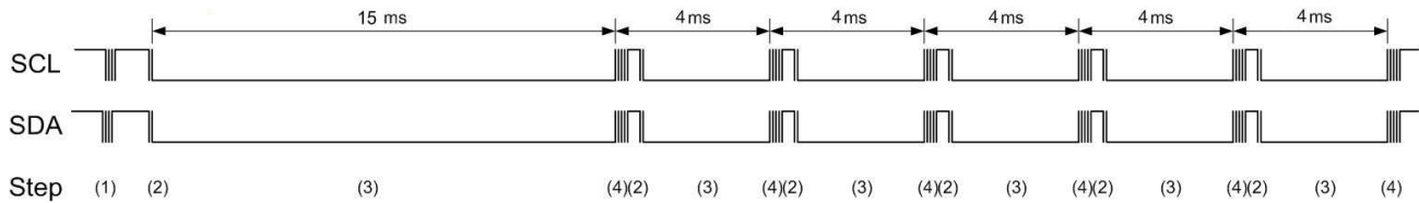
Figure 7. Consecutive blocking read operation steps
