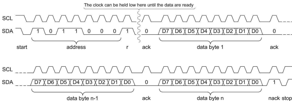
Figure 6. I 2 C read data sequence
