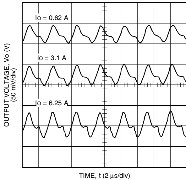
Figure 5. Typical JAW075B1 Output Ripple Voltage at Room Temperature and 48 Vdc Input
