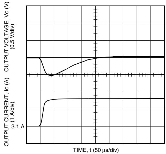
Figure 7. Typical JAW075B1 Transient Response to Step Increase in Load from 50% to 75% of Full Load at Room Temperature and 48 Vdc Input (Waveform Averaged to Eliminate Ripple Component.)
