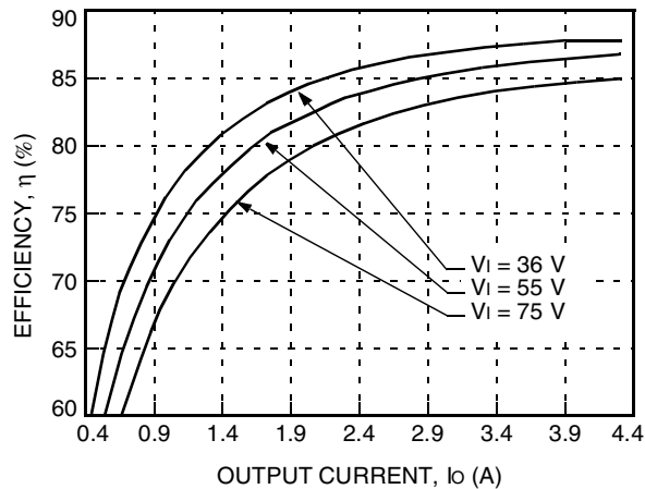
Figure 3. Typical JAW050B1 Efficiency vs. Output Current at Room Temperature
