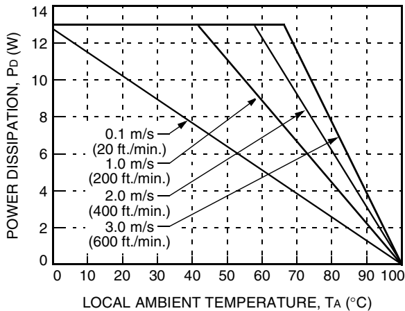
Figure 21. Forced Convection Power Derating with No Heat Sink; Either Orientation
