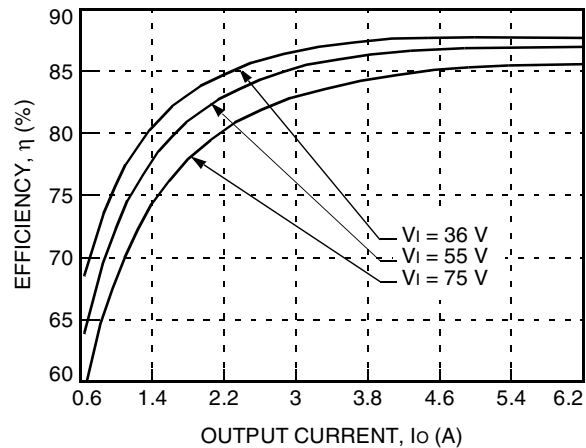
Figure 4. Typical JAW075B1 Efficiency vs. Output Current at Room Temperature
