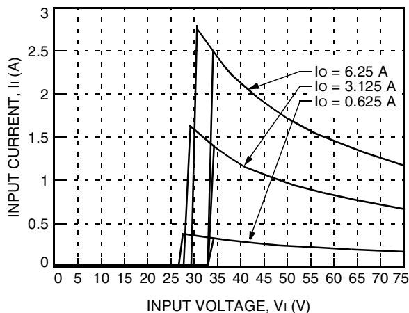
Figure 2. Typical JAW075B1 Input Characteristics at Room Temperature
