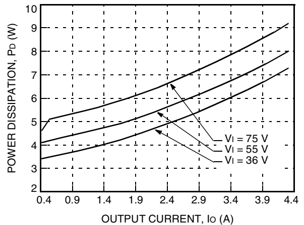
Figure 19. JAW050B1 Power Dissipation vs. Output Current
