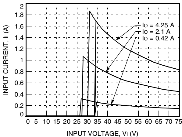
Figure 1. Typical JAW050B1 Input Characteristics at Room Temperature
