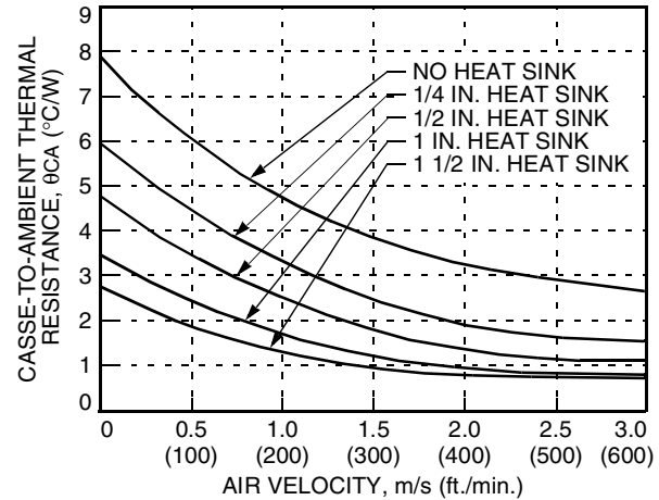
Figure 22. Case-to-Ambient Thermal Resistance Curves; Either Orientation
