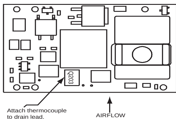
Figure 43. HW/HC 6.6A-12A-Series Temperature Measurement Location (Top View).
