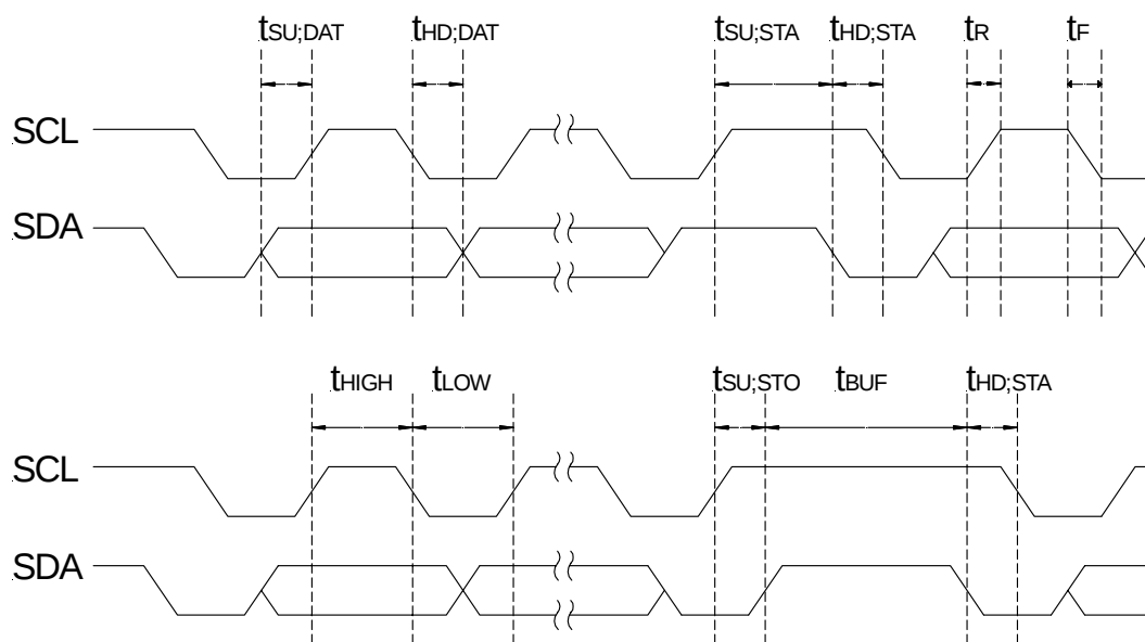
Fig. 2: Timing characteristics
