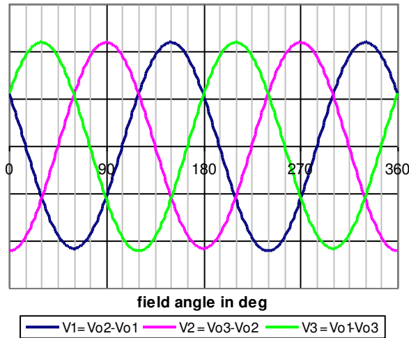
Figure 3: output voltages
