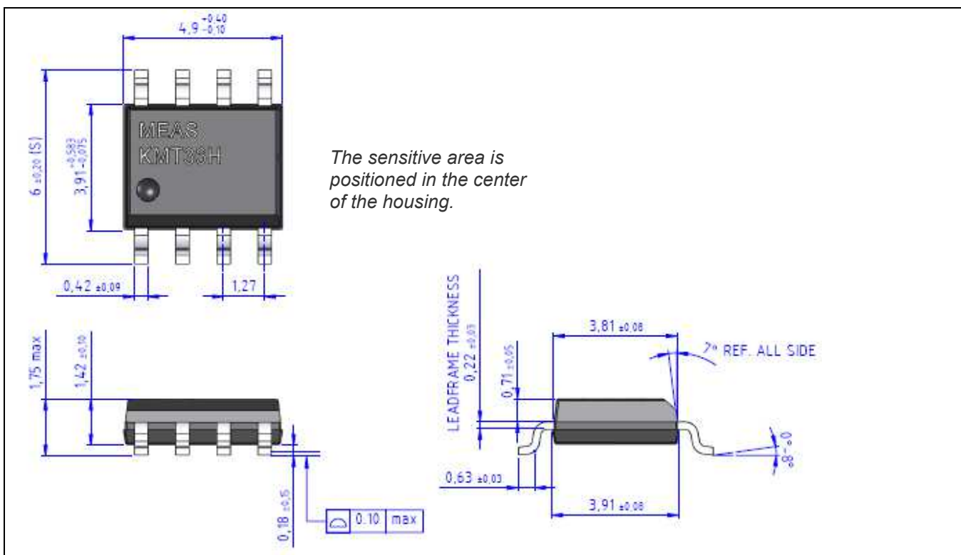
Figure 2: SO8 outline
