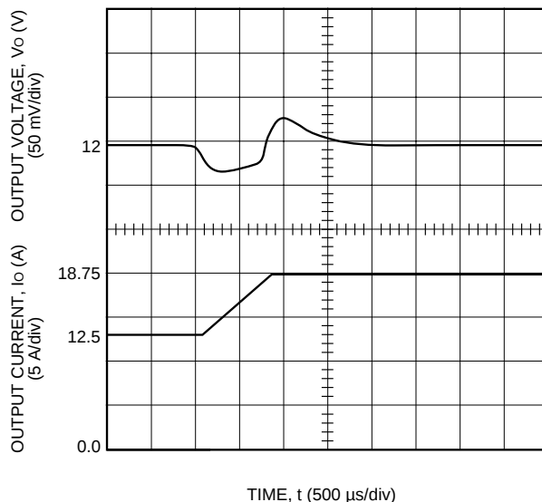
Figure 6. Typical FW300B1 Transient Response to Step Increase in Load from 50% to 75% of Full Load at Room Temperature and 48 V Input (Waveform Averaged to Eliminate Ripple Component.)
