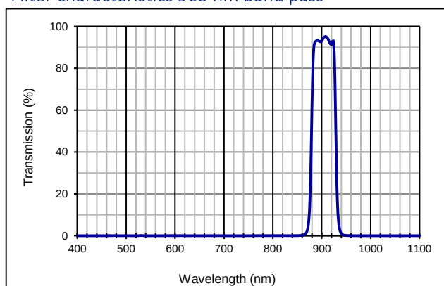
Filter characteristics 905 nm band pass
