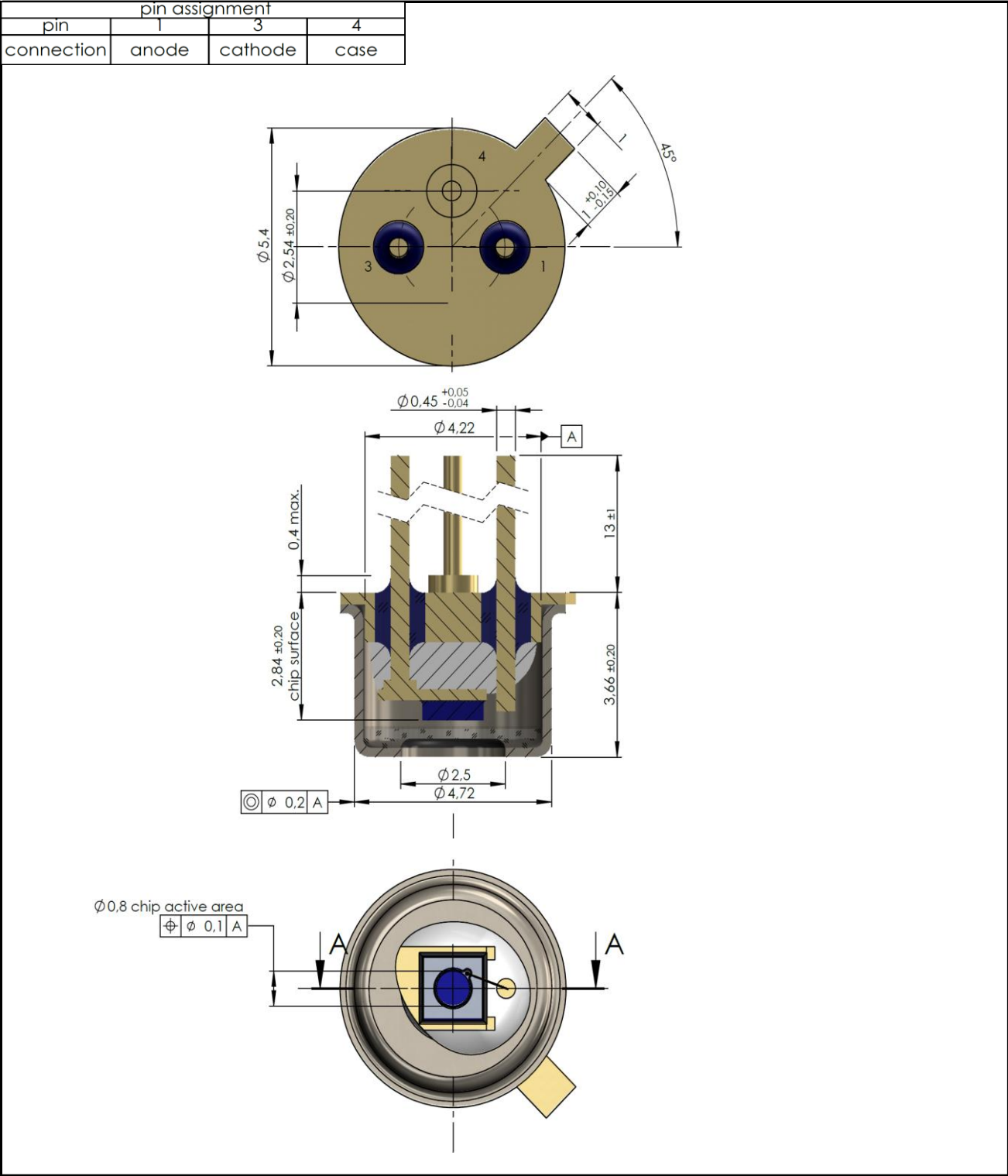
Technical Drawing, Package: TO52
