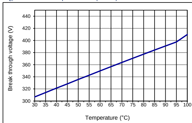
U_{br} as fct of temperature (23 °C)
