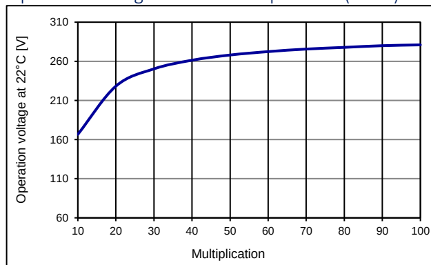
Operation voltage as fct of multiplication (23 °C)
