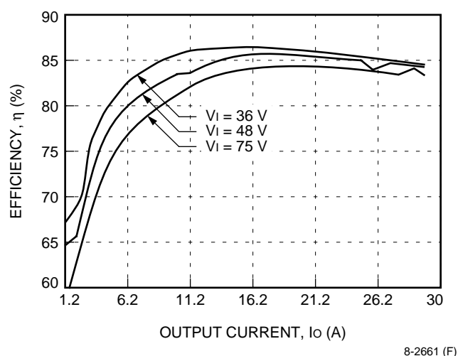
Figure 3. Typical FW300S10R01 Efficiency vs. Output Current at Room Temperature
