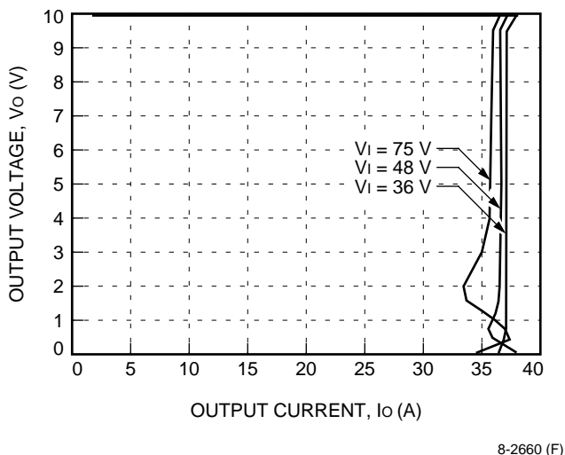
Figure 2. Typical FW300S10R01 Output Characteristics at Room Temperature
