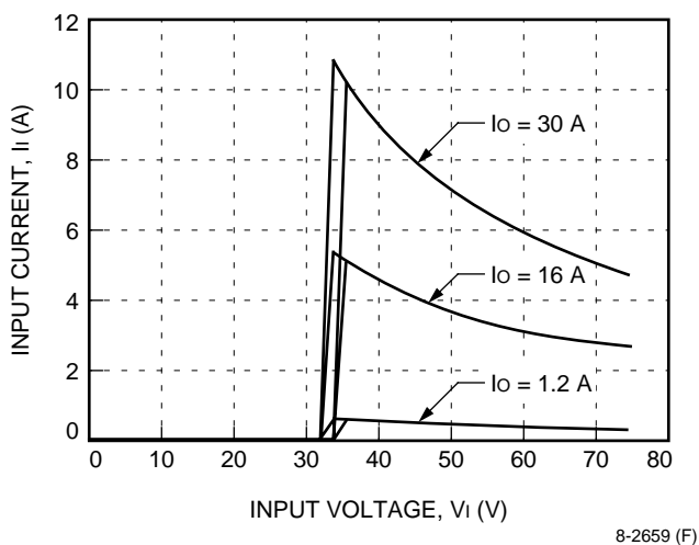
Figure 1. Typical FW300S10R01 Input Characteristics at Room Temperature
