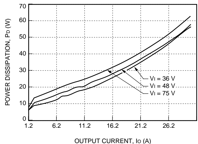
Figure 23. FW300S10R01 Power Dissipation vs. Output Current
