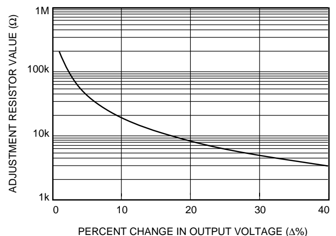
Figure 14. Resistor Selection for Decreased Output Voltage
