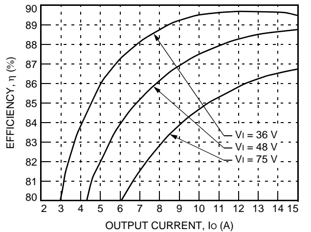
Figure 5. Typical JAHW075F Converter Efficiency vs. Output Current at Room Temperature
