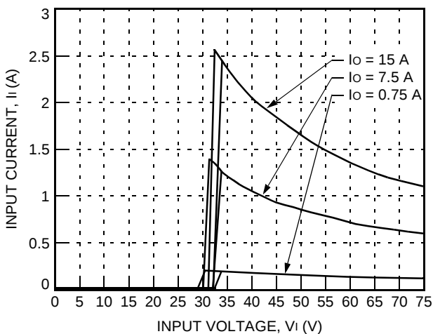
Figure 2. Typical JAHW075A Input Characteristics at Room Temperature
