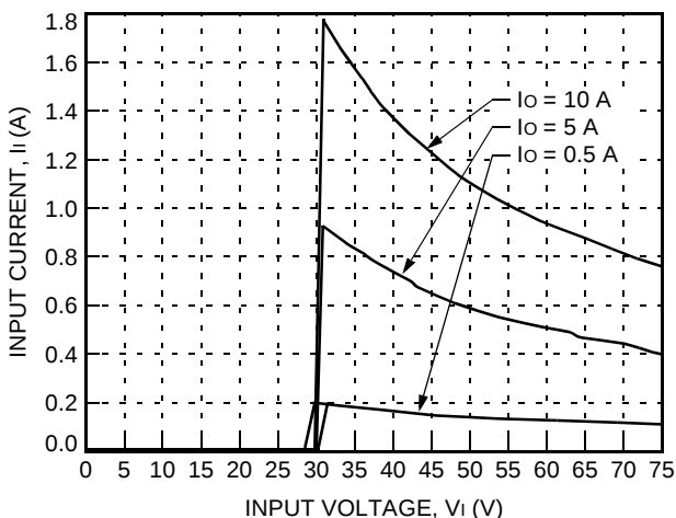
Figure 1. Typical JAHW050A Input Characteristics at Room Temperature
