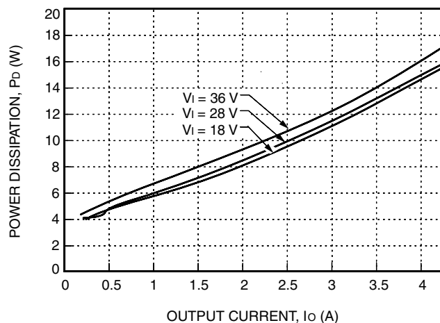
Figure 24. JC100H Power Dissipation vs. Output Current
