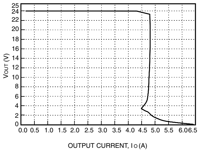
Figure 6. Typical JC100H Output Characteristics at Room Temperature, V_{IN} = 28 V
