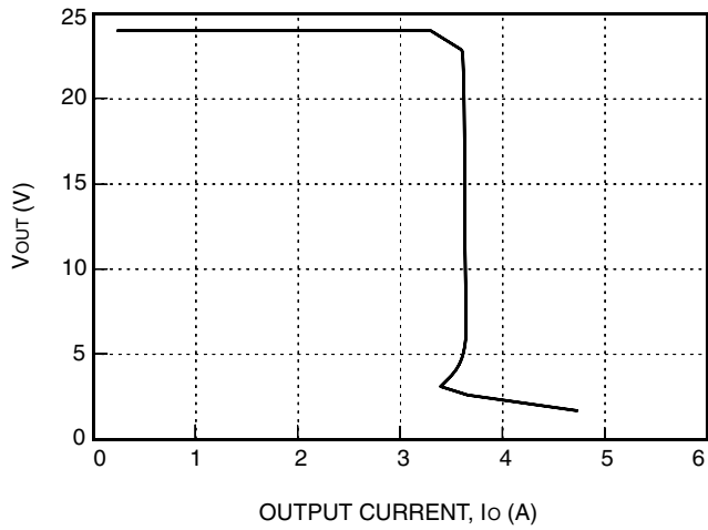
Figure 5. Typical JC075H Output Characteristics at Room Temperature, V_{IN} = 28 V
