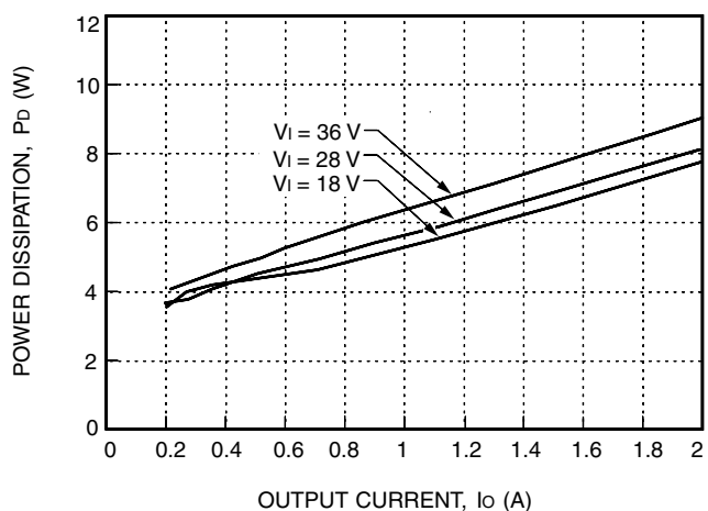
Figure 22. JC050H Power Dissipation vs. Output Current
