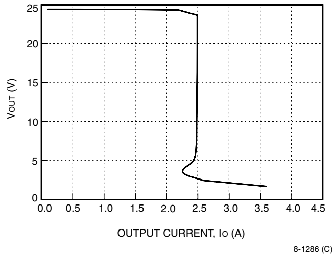
Figure 4. Typical JC050H Output Characteristics at Room Temperature, V_{IN} = 28 V
