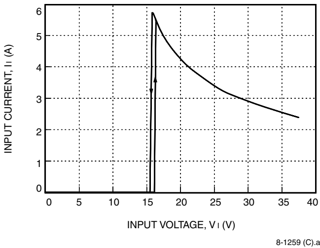
Figure 2. Typical JC075H Input Characteristics at Room Temperature, I_o = 3.1 A
