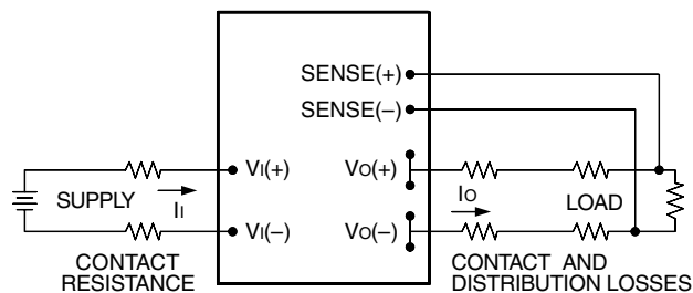
Figure 15. Effective Circuit Configuration for Single-Module Remote-Sense Operation
