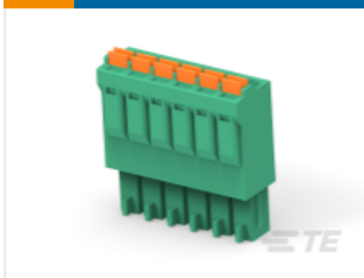
TE Part #2350398-6 6 POS SPRING TB PLUG , PITCH 3.50
