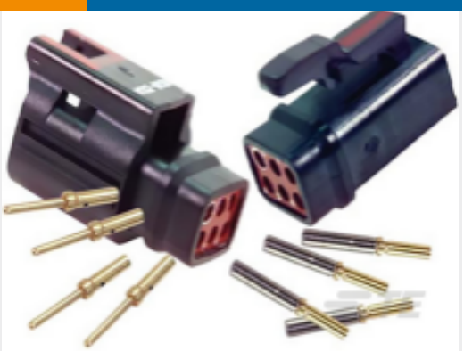
TE Part #ASC605-06PD PLUG.AS MODULAR.PIN.
