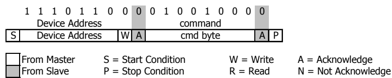
Figure 9: I2C command to initiate a pressure conversion (OSR=4096, typ=D1)
