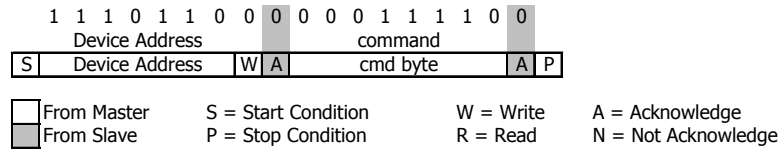
Figure 6: I2C Reset Command
