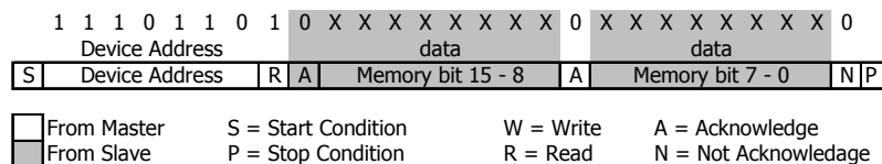
Figure 8: I2C answer from MS5837-07BA
