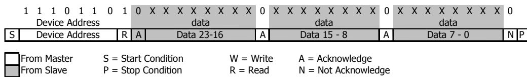
Figure 11: I2C answer from MS5837-07BA
