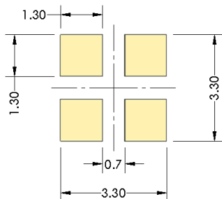
Figure 15: PCB footprint
