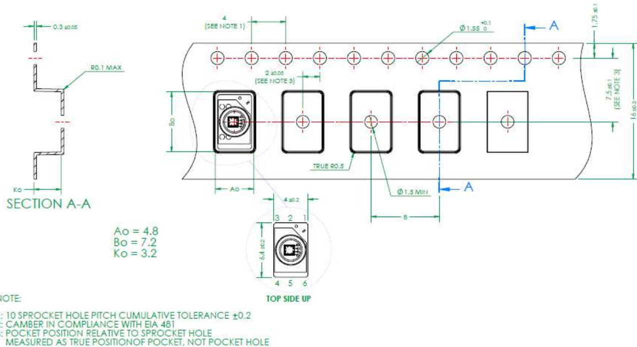
Figure 20: Tape & reel
