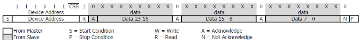
Figure 6: I 2 C pressure response (D1) on 24 bit from MS5803-30BA
