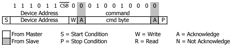
Figure 4: I 2 C Command to initiate a pressure conversion (OSR=4096, typ=D1)
