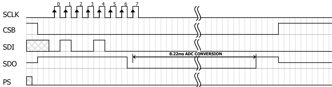
Figure 11: Conversion out sequence, Typ=d1, OSR = 4096
