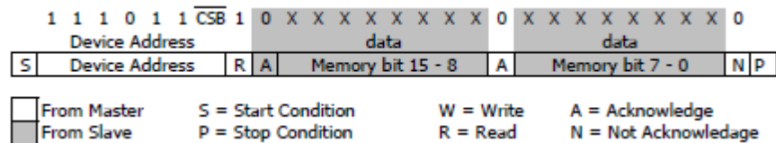
Figure 8: I 2 C answer from MS5803-30BA
