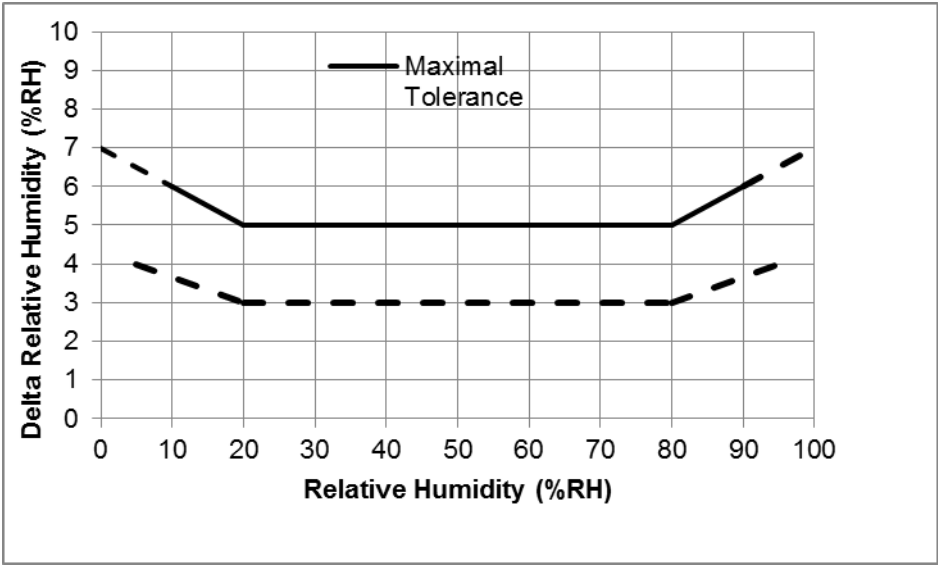
GRAPH 1: RELATIVE HUMIDITY ERROR BUDGET CONDITIONS AT 25°C
