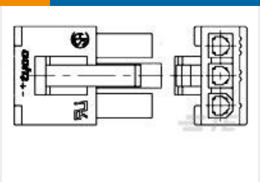
TE Part #2029112-3 3P RCPT SR VAL-U-LOK GW
