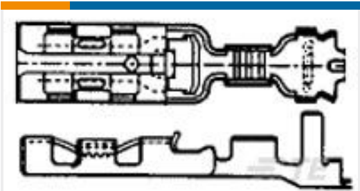
TE Part #353249-2 110 PL EX REC. 26-22AWG PTPHBZ
