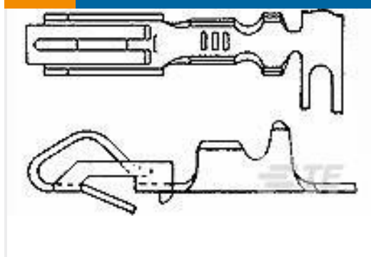
TE Part #3-61668-1 BIF-LEAF CONT CR/SNAP SN/BR
