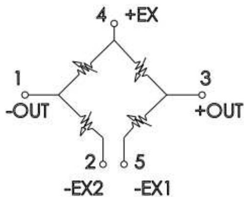
APPLICATION SCHEMATIC
