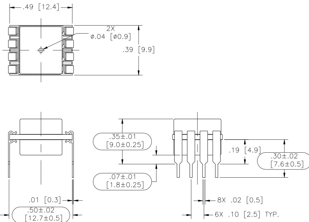
Model: MS4525-MMvxxxxyS
