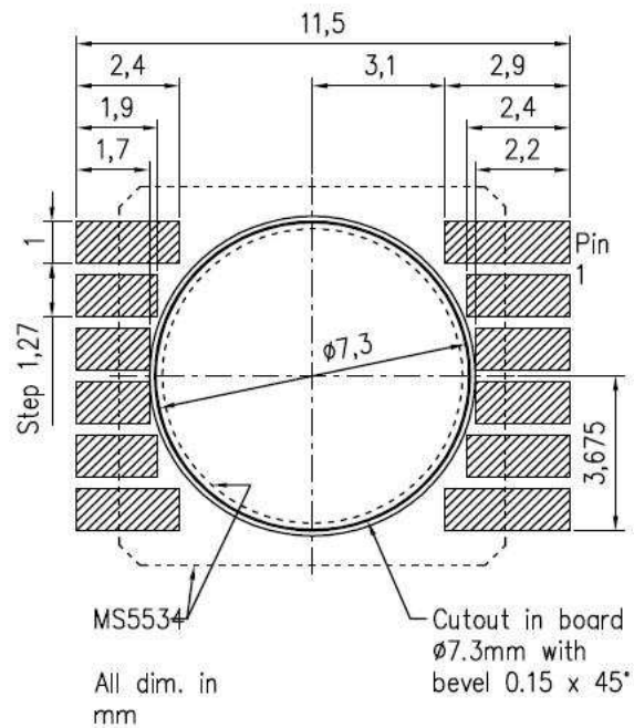
Fig. 10: Layout for topside
