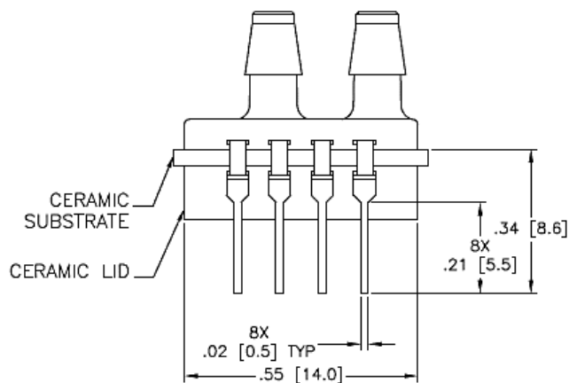
Sensor Pinout
