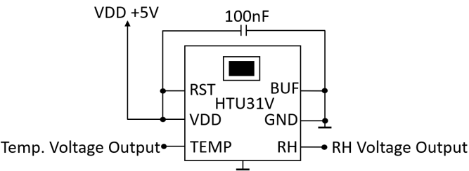
Figure 4 HTU31V Typical Application Circuit
