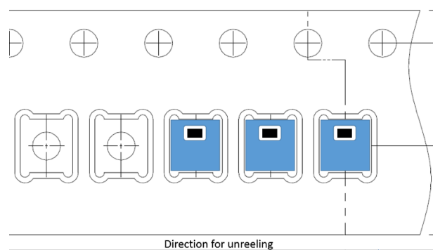
Figure 14 Product Orientation in Tape and Reel Packaging
