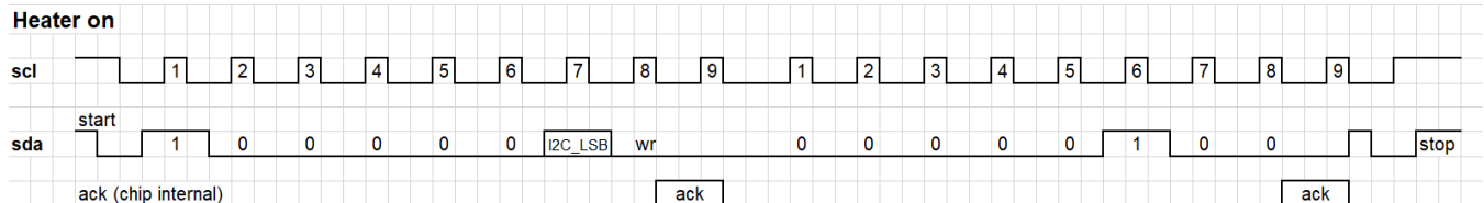
Figure 9 Heater on Command
