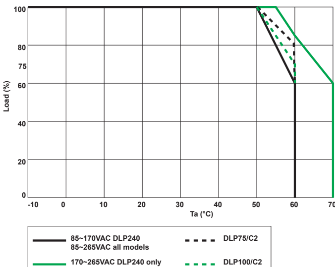
Derating Curve
