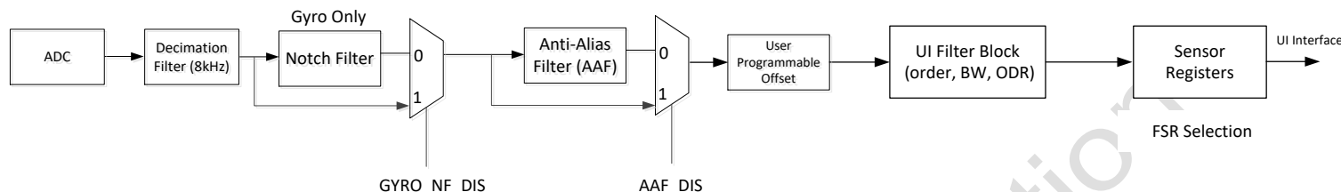
Figure 8. ICM-40608 Signal Path
