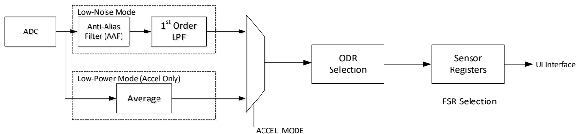
Figure 8. ICM-42370-P Signal Path
