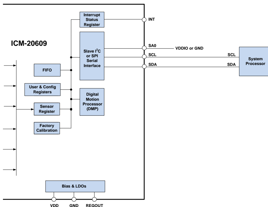
Figure 6. ICM-20609 Solution Using I 2 C Interface
