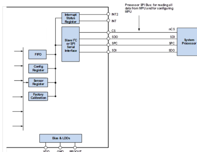
Figure 7. IAM-20381HT Solution Using SPI Interface
