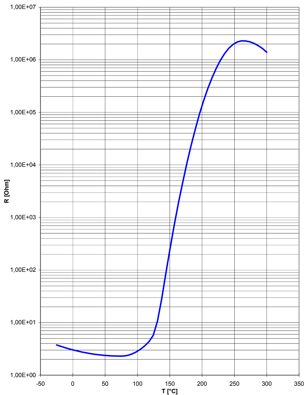
Typ. RT-Curve
